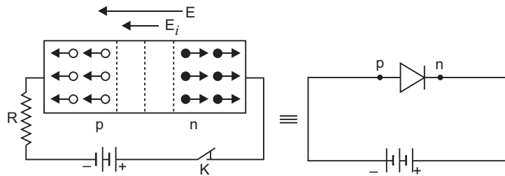
Reverse current
