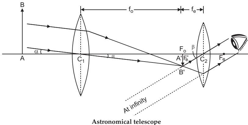
Astronomical telescope
