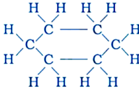
(b) complete molecule
