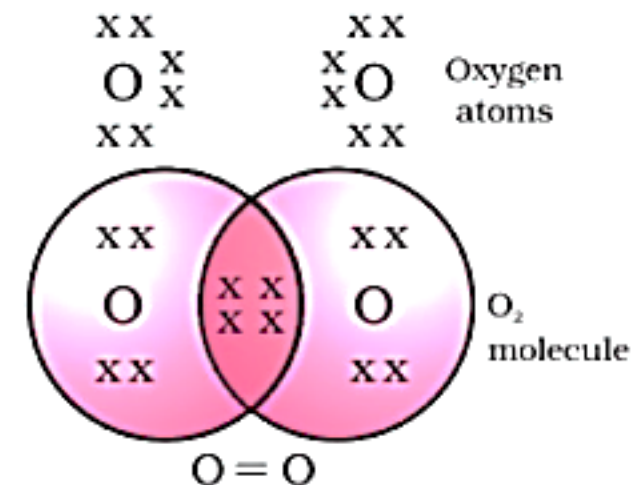
\text{O} = \text{O} Double bond between two oxygen atoms
