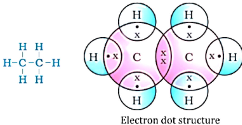
Structure of ethane
