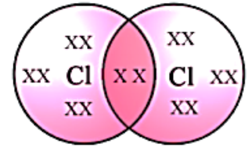
\text{Cl} - \text{Cl} or \text{Cl}_2 molecule
