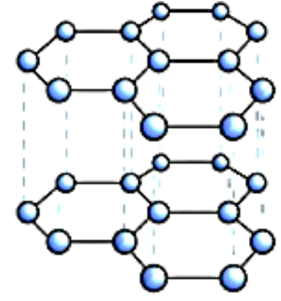
Structure of graphite
