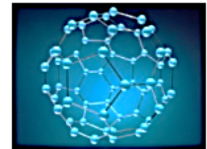
Structure of C-60 Buckminsterfullerene
